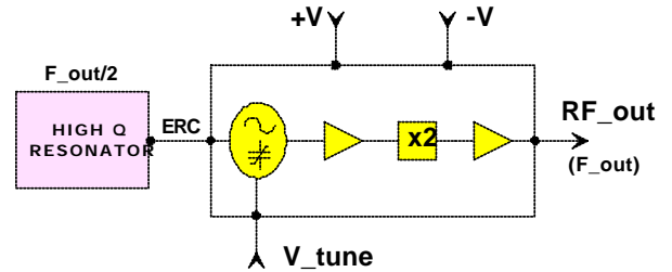
Multifunction block diagram
